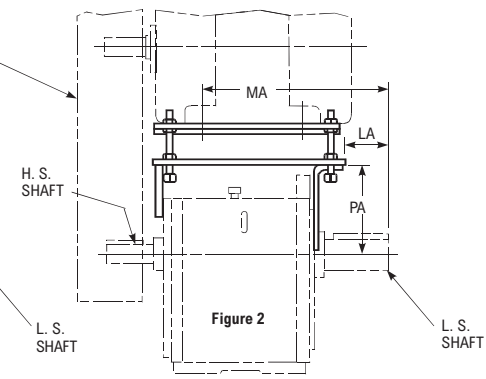
Size 2060-2100 ... 250-400T & U (Size 2060 Max. U-Frame is 404)
