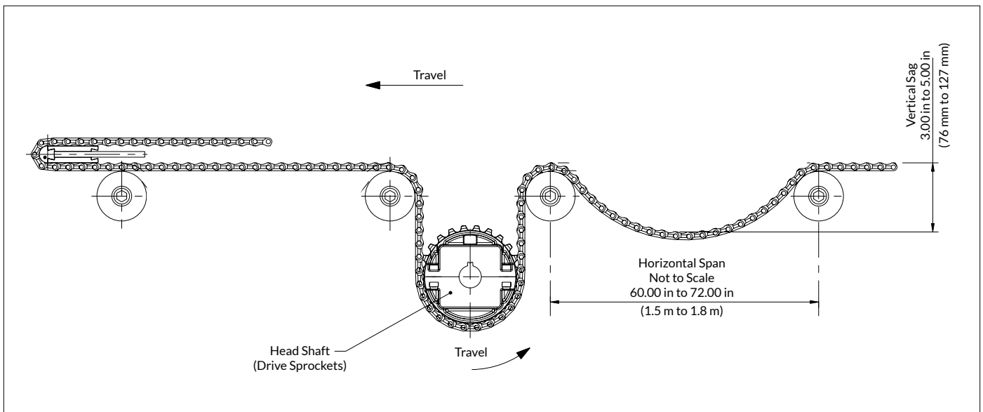
Concept B: Drive Configuration for Uni-Directional Conveyor (Drawing is shown with 1500 Series MatTop Chain)
