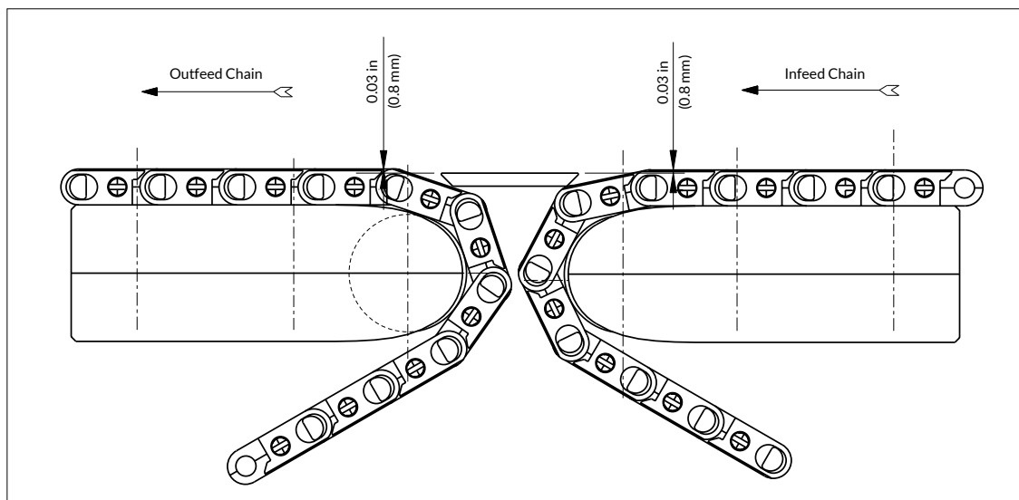
Infeed chain and outfeed chain are level to each other and the transfer plate steps down
