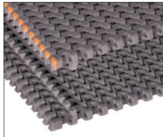
7526 MATTOP CHAIN has a 0.50-inch (12.7 mm) pitch and can be used in side-flexing applications
