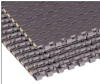
1500 MATTOP CHAIN has a 0.59-inch (15 mm) pitch and curved bottom contour
