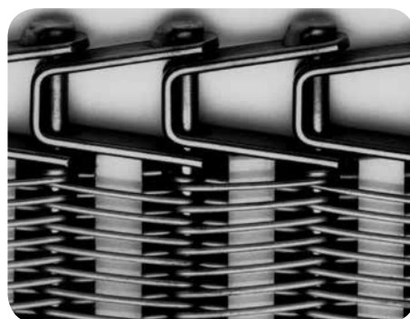
Cam-Grid® with filler strips.
