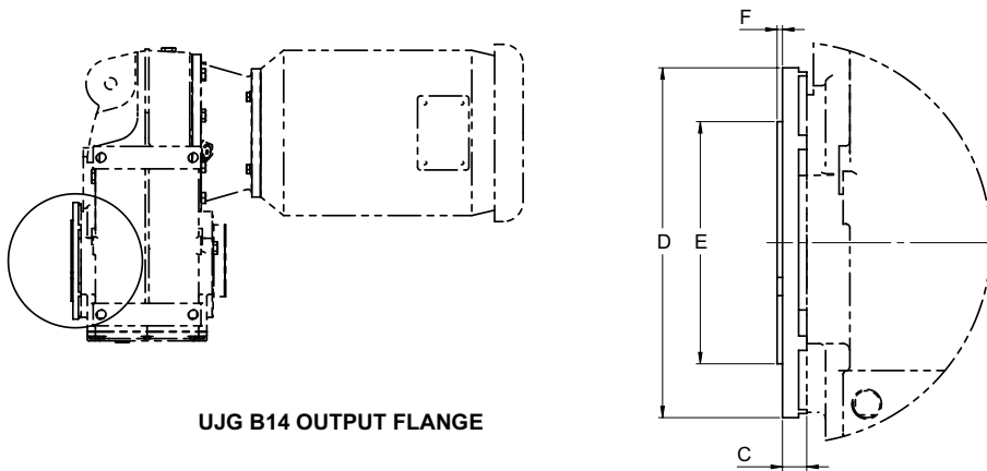
B14 Output Flange — 300UJG (Dimensions—Inch)
